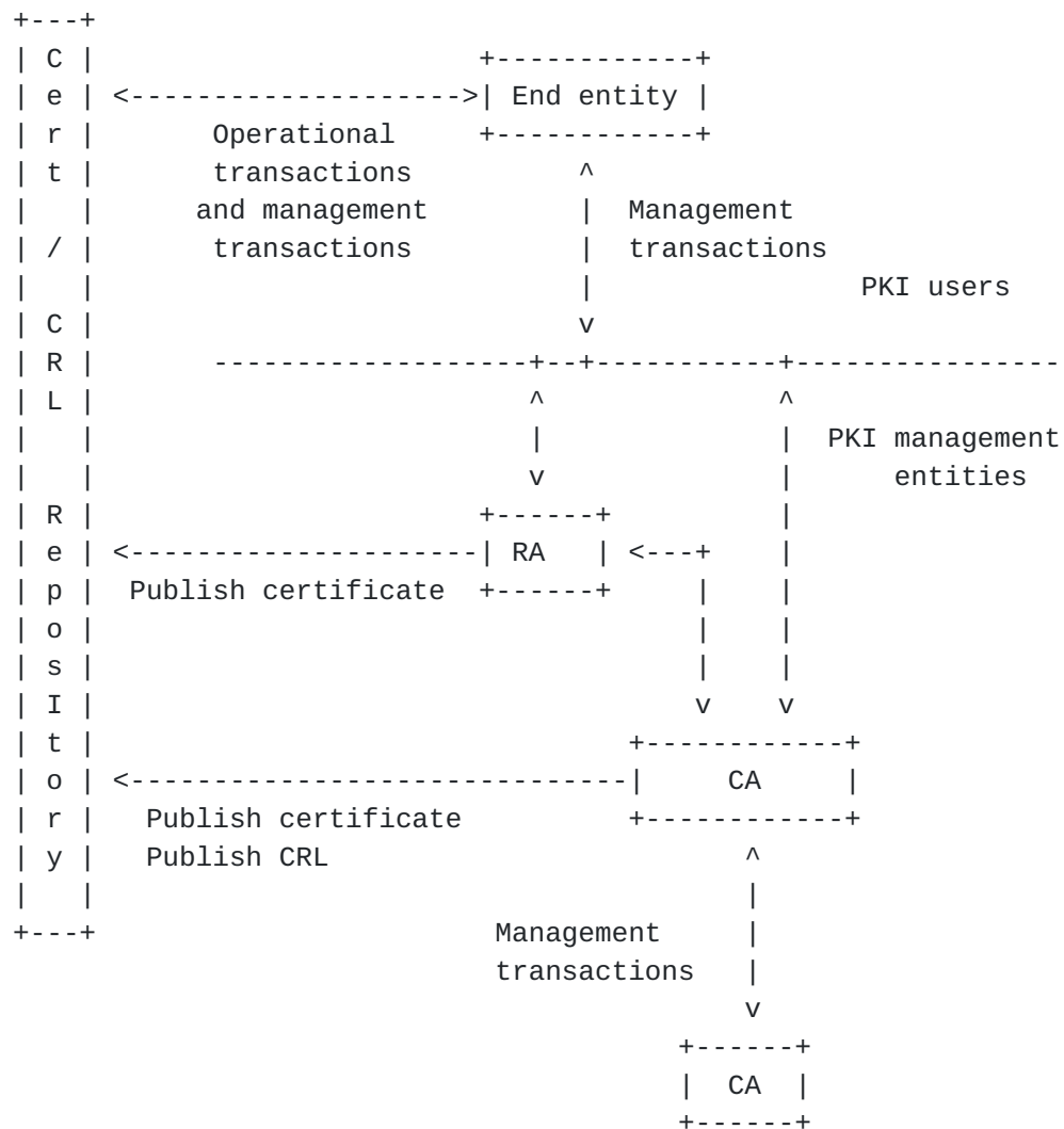
Figure 1 - PKI Entities
